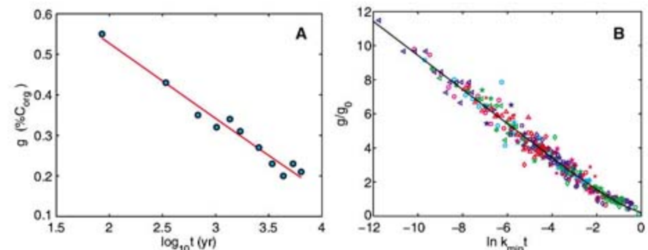
Fig. 2. (A) Concentration (weight %) of organic carbon (filled circles) from Pacific-Antarctic Ridge sediment core 7812-05 of Reimers and Suess (32). The theoretical curve (smooth line) corresponds to Eq. 2 with \log_{10} k_{\min} \cong -5.1 ( \text{year}^{-1} ) and g_0 = 0.08 ( \%C_{\text{org}} ). (B) Rescaling of 23 cores (287 points total) with respect to dimensionless axes \ln k_{\min} t and g/g_0 . Each core corresponds to a different k_{\min} , g_0 pair. Different colors and symbols correspond to different cores. Red corresponds to cores underlying anoxic environments.
